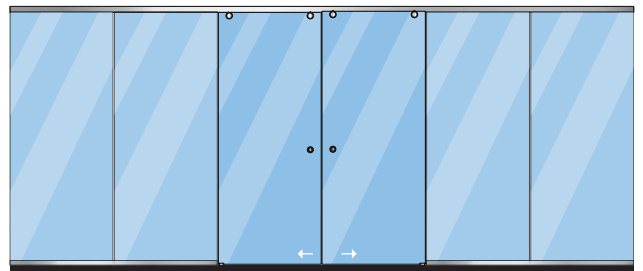
OOOXO-DOUBLE DOOR & TWO SIDELITES ON EACH SIDE
