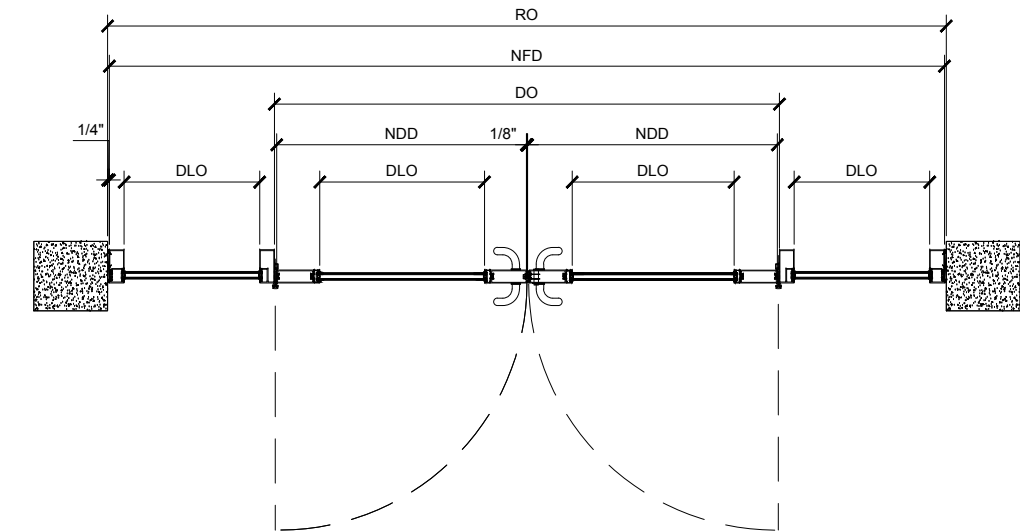
⑥ PLAN VIEW STOREFRONT (PAIR) ARCH REF: SCALE: 1"=1'-0"
