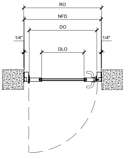
④ PLAN VIEW (SINGLE) ARCH REF: SCALE: 1"=1'-0"
