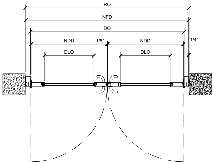
⑤ PLAN VIEW (PAIR) ARCH REF: SCALE: 1"=1'-0"
