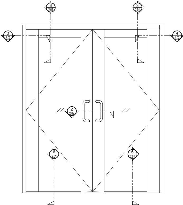
② ELEVATION (PAIR) ARCH REF: SCALE: 1"=1'-0"
