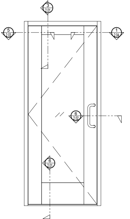
① ELEVATION (SINGLE) ARCH REF: SCALE: 1"=1'-0"
