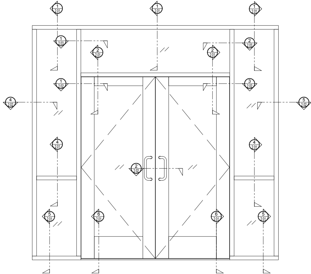
③ ELEVATION STOREFRONT (PAIR) ARCH REF: SCALE: 1"=1'-0"
