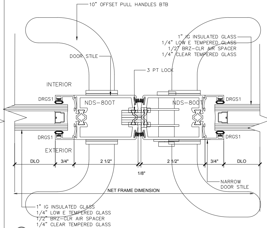
② DOOR STILES (@DOOR) ARCH REF: SCALE: 1'-0"=1'-0"
