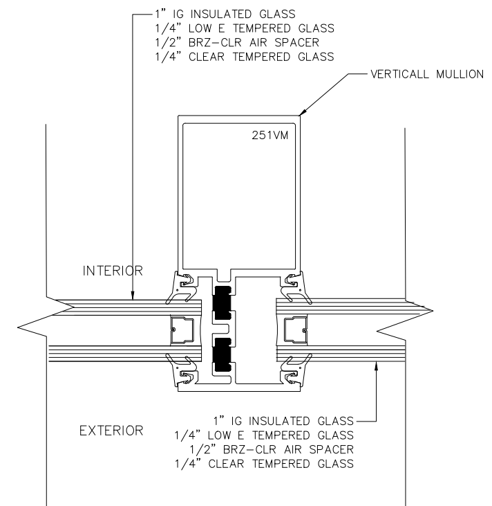
⑥ TRANSOM & SIDELITE (@VYNIL SASH) ARCH REF: SCALE: 1'-0"=1'-0"
