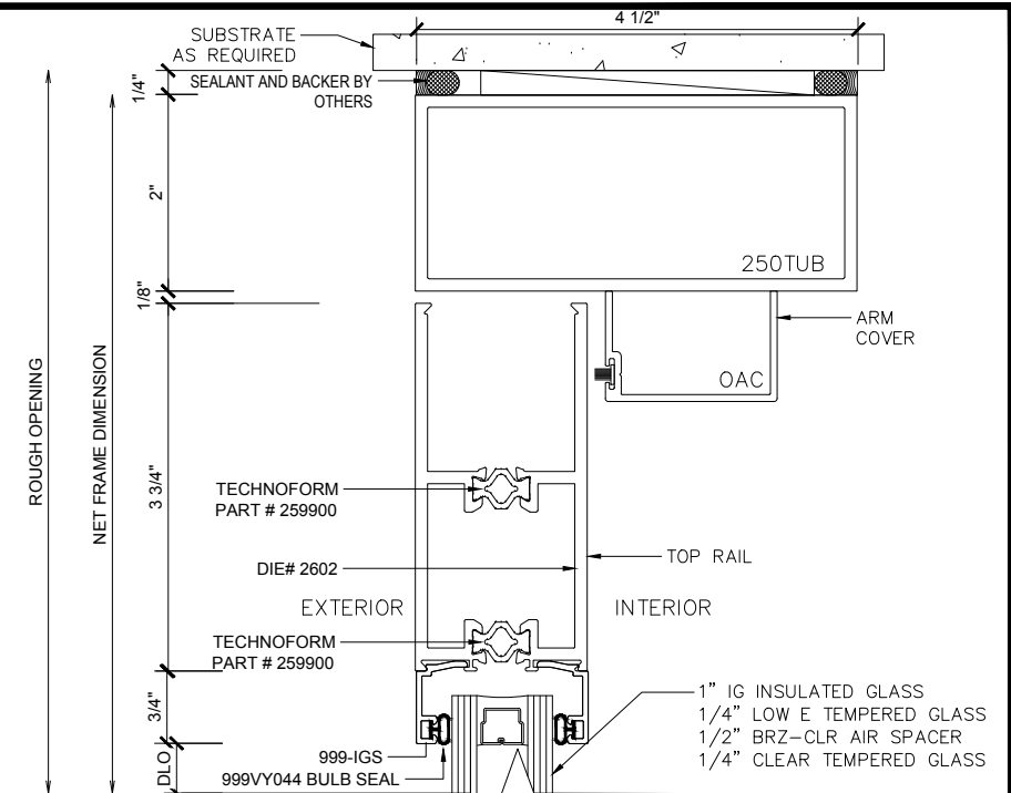
③ TOP RAIL (@DOOR) ALUMINUM DOOR SCALE: 1'-0" = 1'-0"
