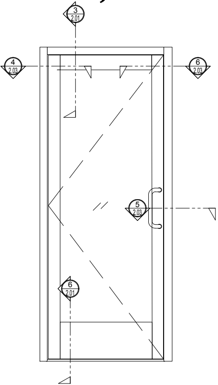
① ELEVATION (SINGLE) ARCH REF: SCALE: 1"=1'-0"
