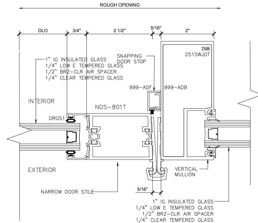
③ JAMB & SIDELITE (@STOREFRONT PAIR DOORS) HINGE: GEAR HINGE SCALE: 1'-0"=1'-0"
