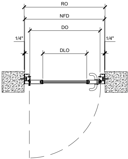
④ PLAN VIEW (SINGLE)
