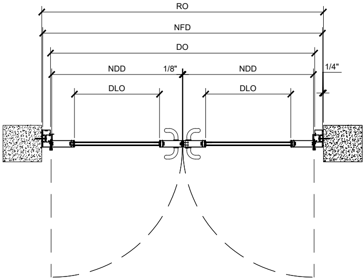
⑤ PLAN VIEW (PAIR)
