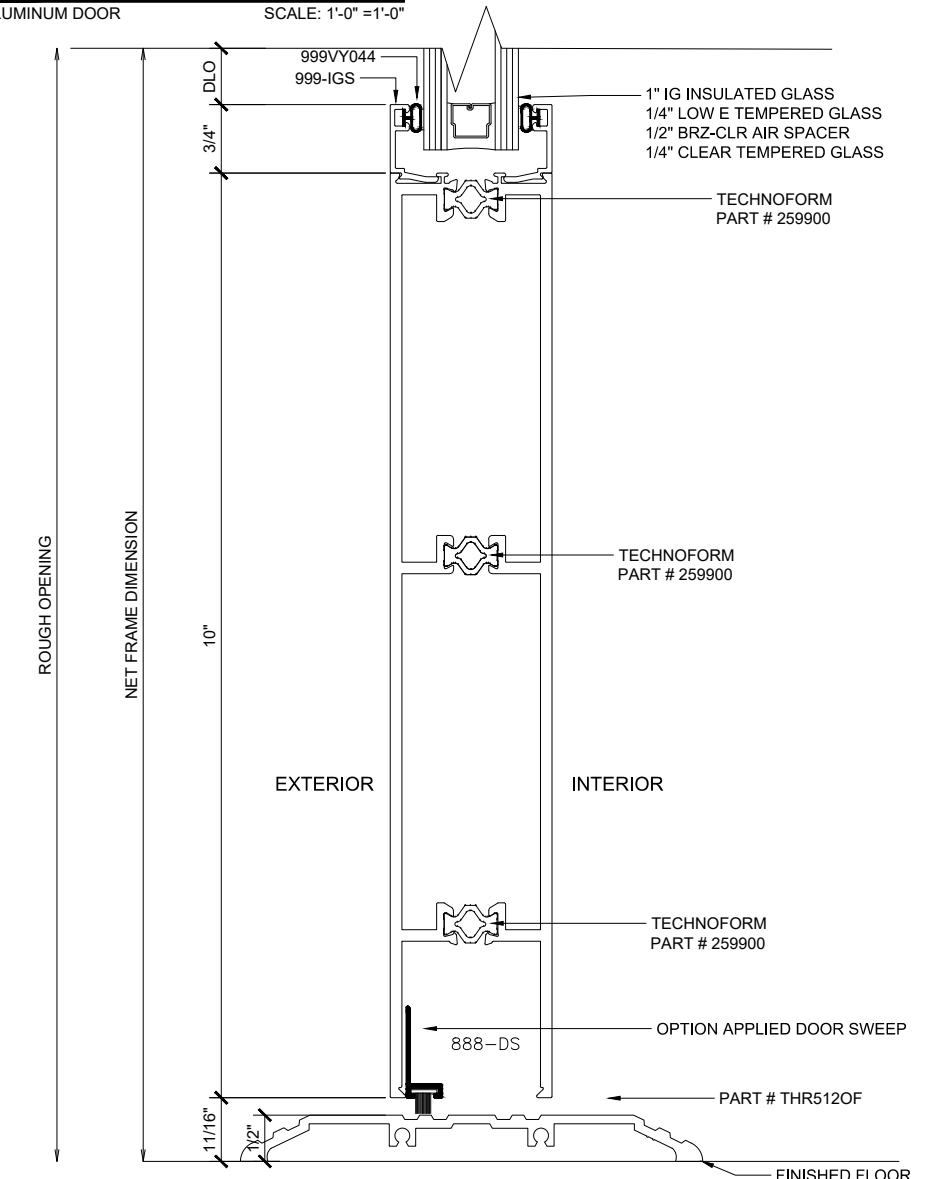
⑥ BOTTOM RAIL (@DOOR) ALUMINUM DOOR SCALE: 1'-0" = 1'-0"
