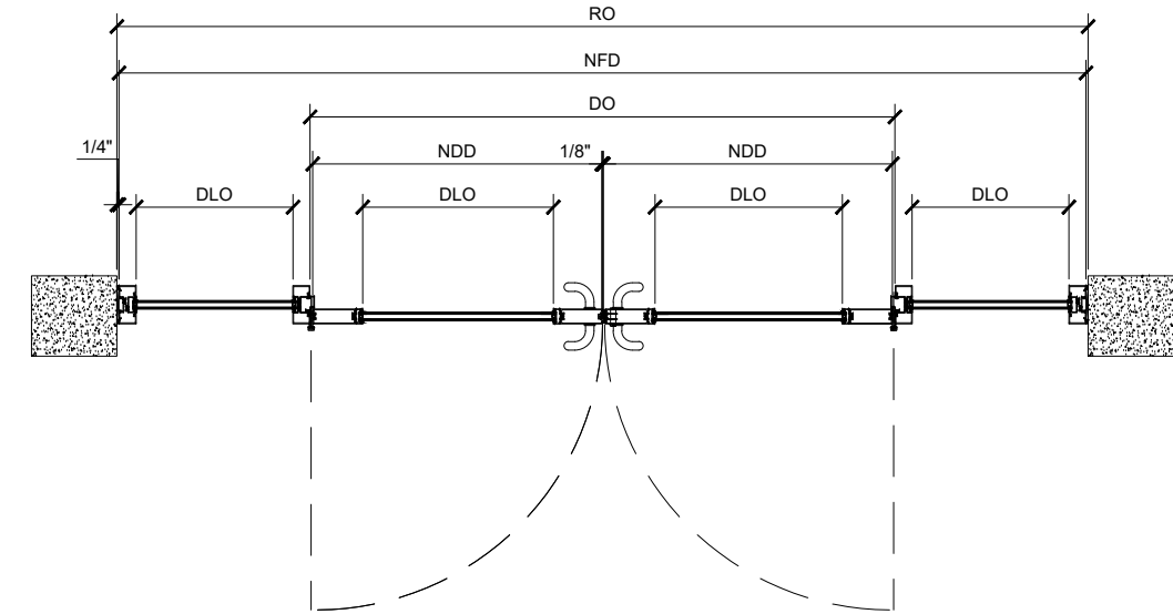
⑥ PLAN VIEW STOREFRONT (PAIR)
