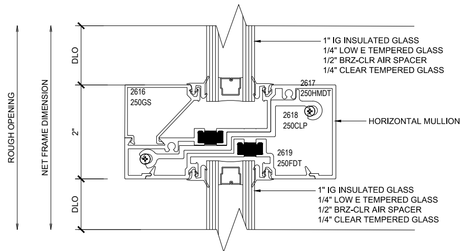
④ VERTICAL MULLION (@SIDELITE) STOREFRONT SIDELITE SCALE: 1'-0" = 1'-0"
