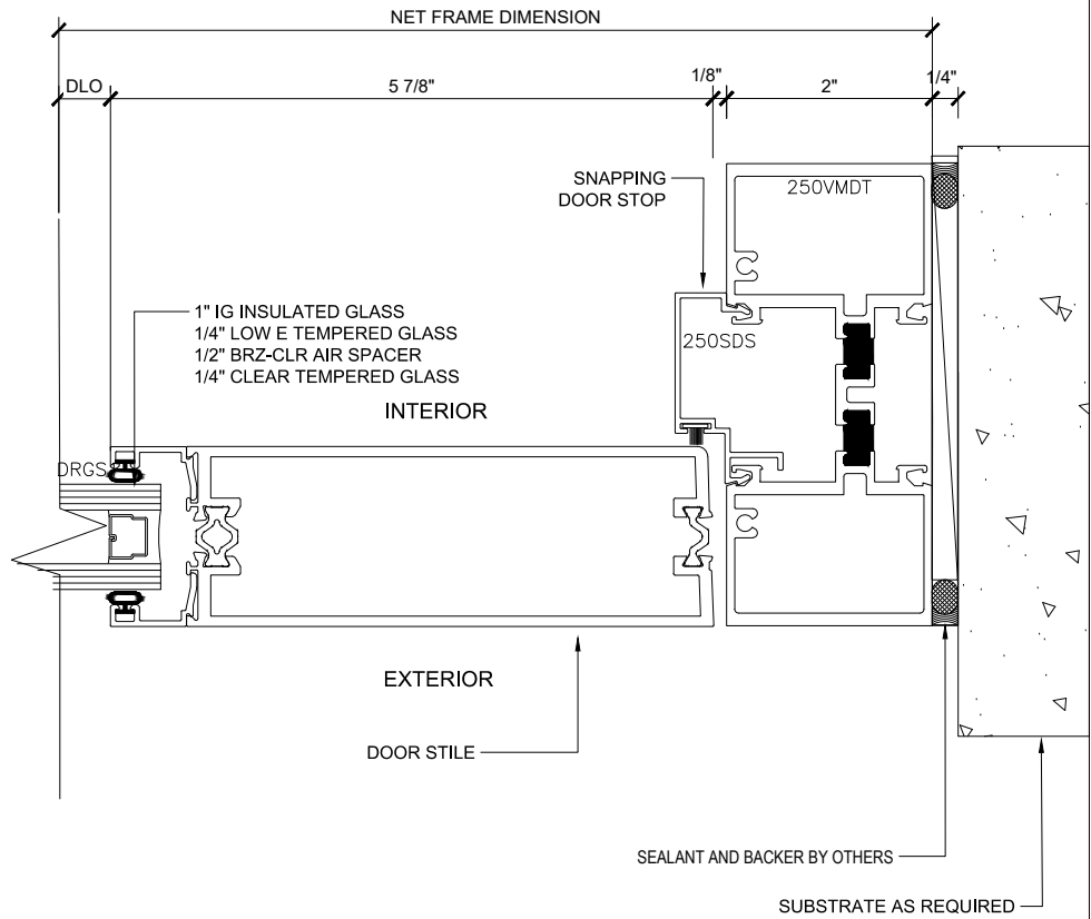
① JAMB (@ SINGLE DOOR) HINGE: GEAR HINGE SCALE: 1'-0"=1'-0"
