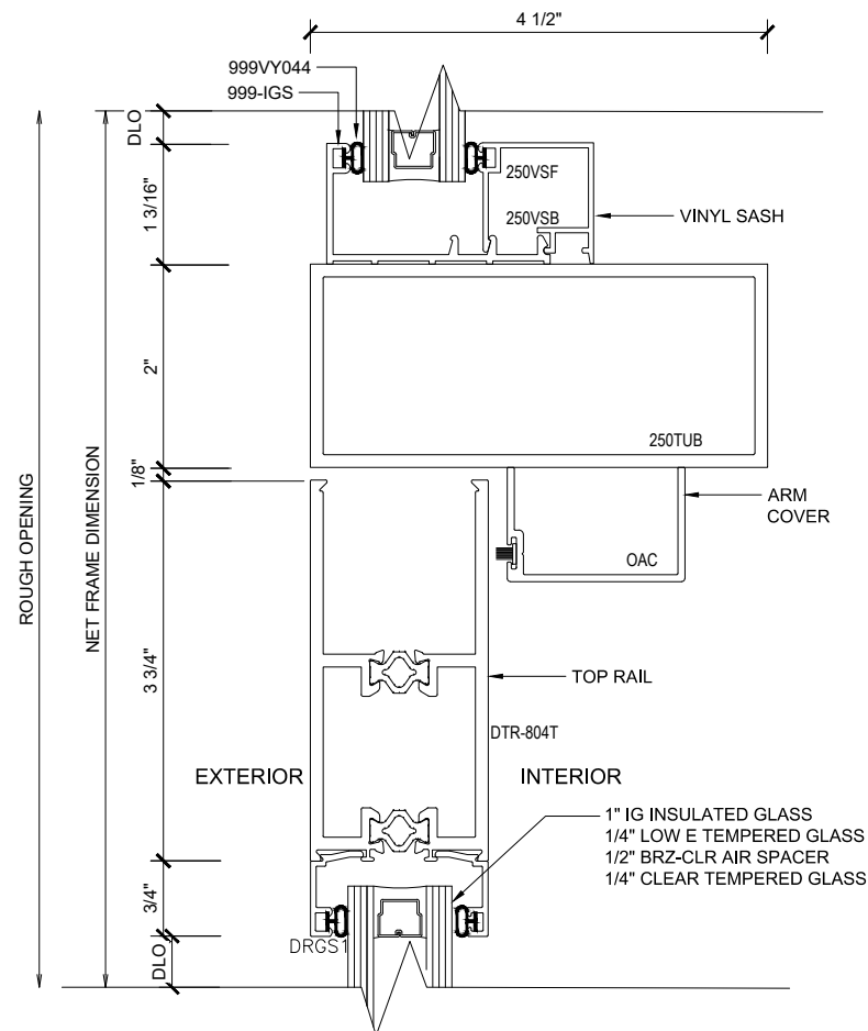
② TOP RAIL & TRANSOM (@DOOR) ALUMINUM DOOR SCALE: 1'-0" = 1'-0"
