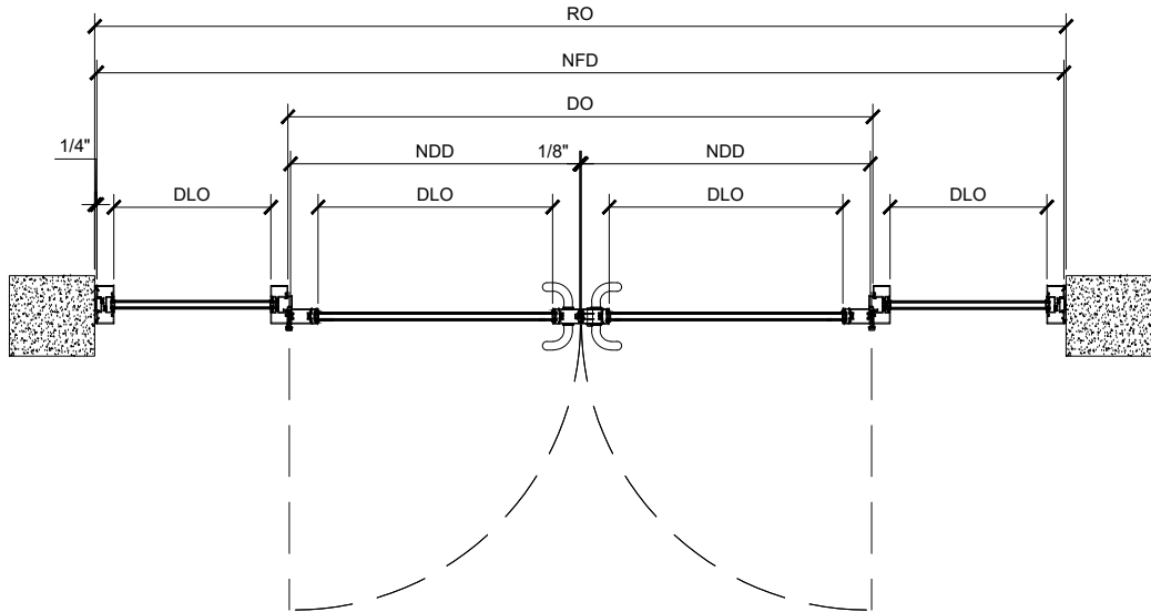
6 PLAN VIEW STOREFRONT (PAIR)
