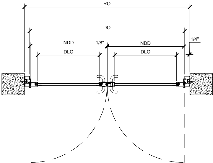
5 PLAN VIEW (PAIR)
