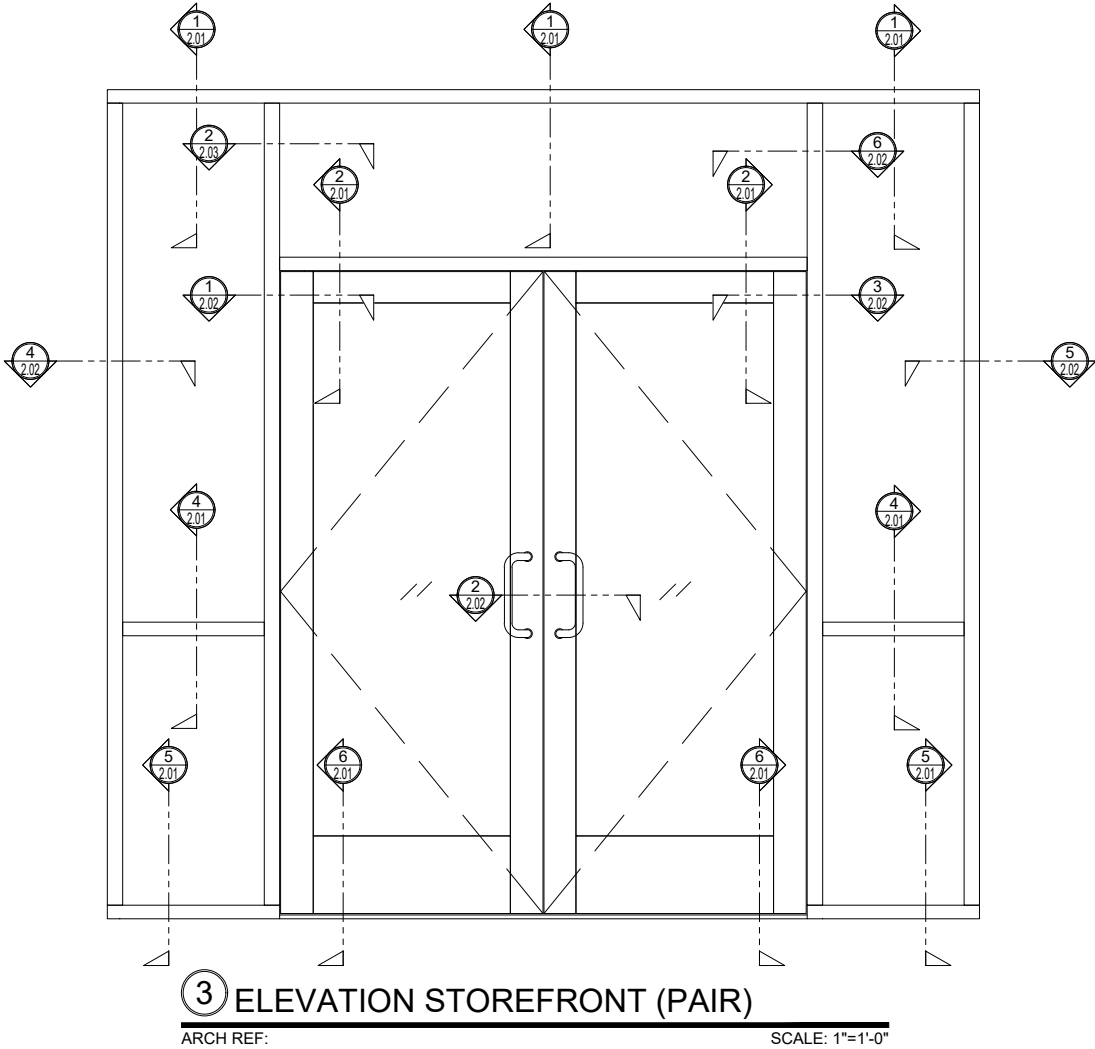
② ELEVATION (PAIR) ARCH REF: SCALE: 1"=1'-0"
