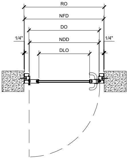
④ PLAN VIEW (SINGLE) ARCH REF: SCALE: 1"=1'-0"
