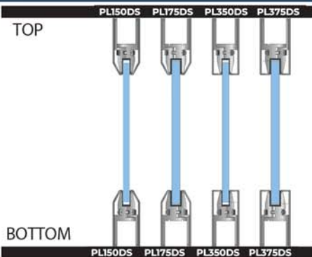
SINGLE DOOR
