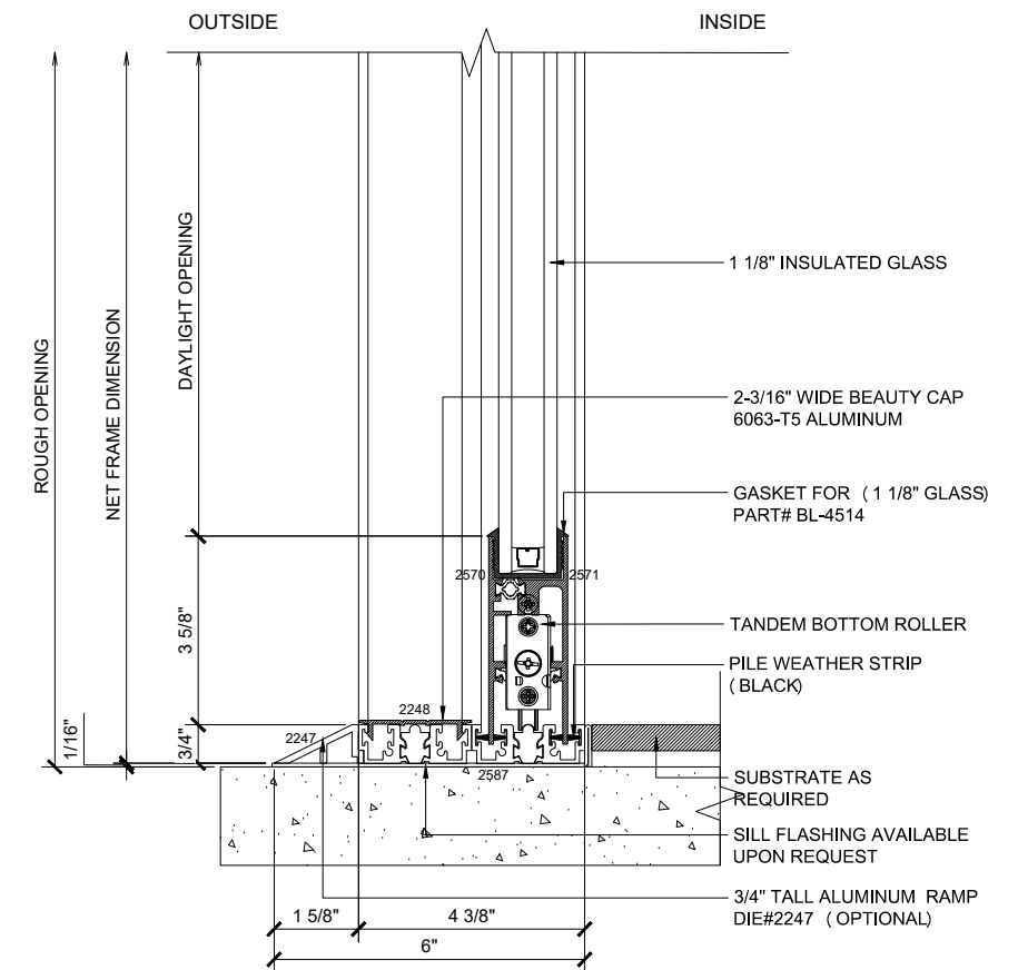
④ SILL (@SLIDER)
