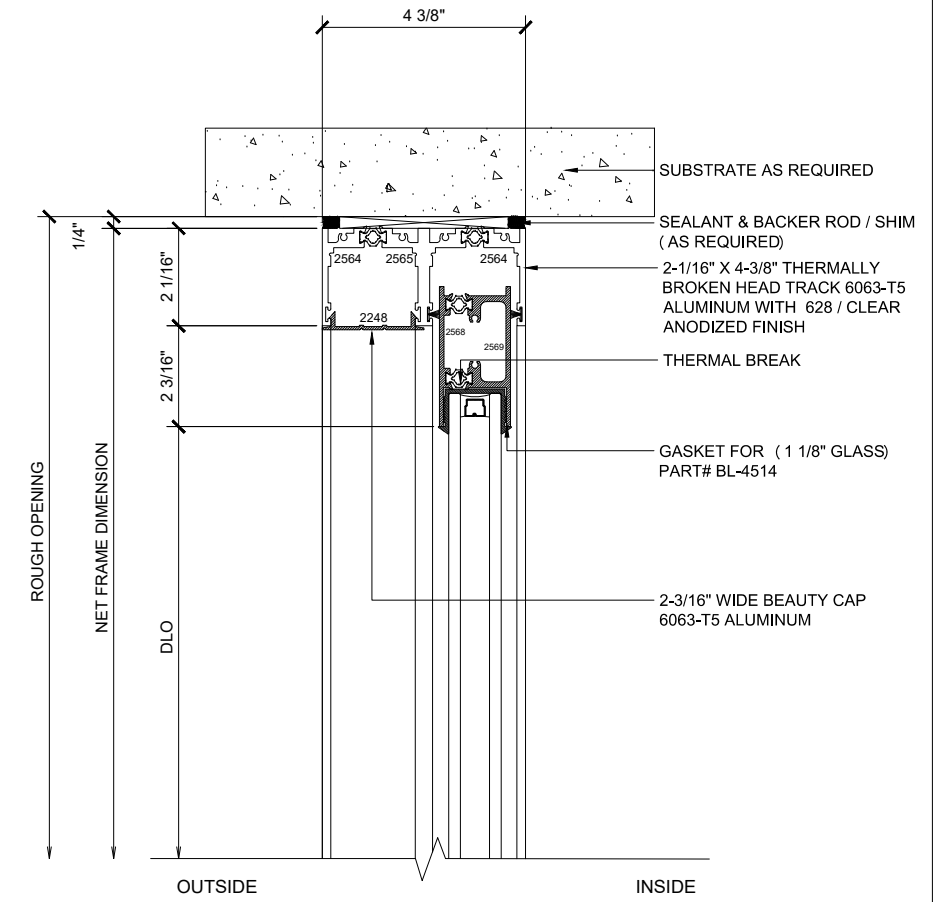
③ HEAD (@SLIDER)
