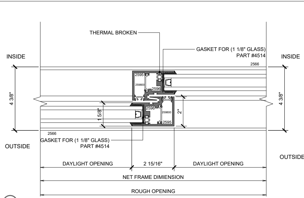
② VERTICAL
