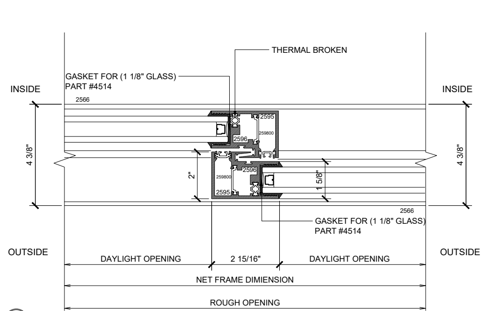
⑤ VERTICAL
