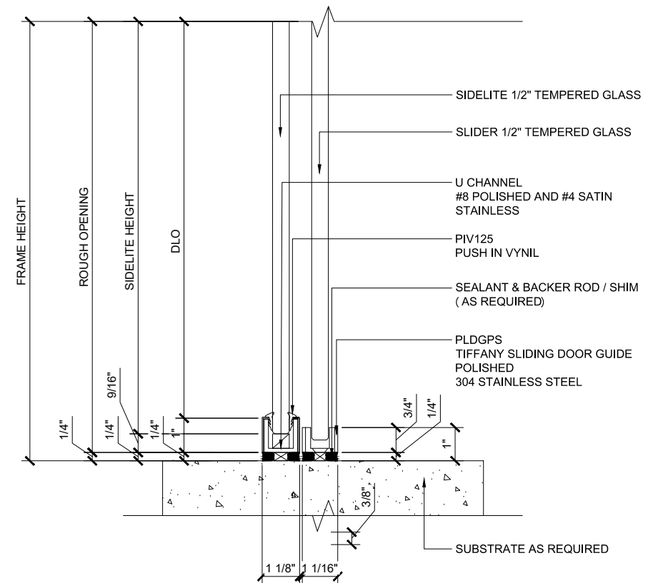
④ SILL (@SIDELITE)
