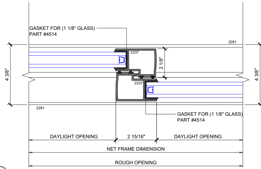
② VERTICAL
