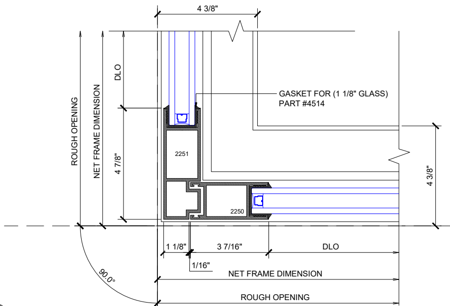
④ 90° CORNER DETAIL
