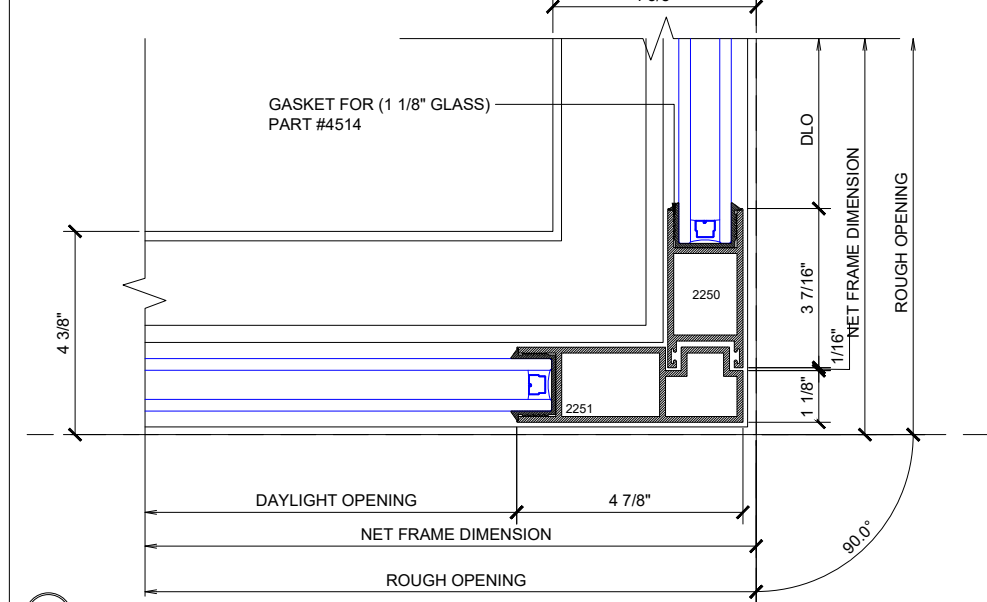
③ 90° CORNER DETAIL
