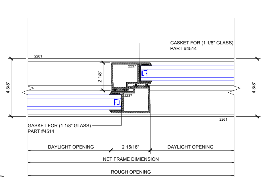
⑤ VERTICAL
