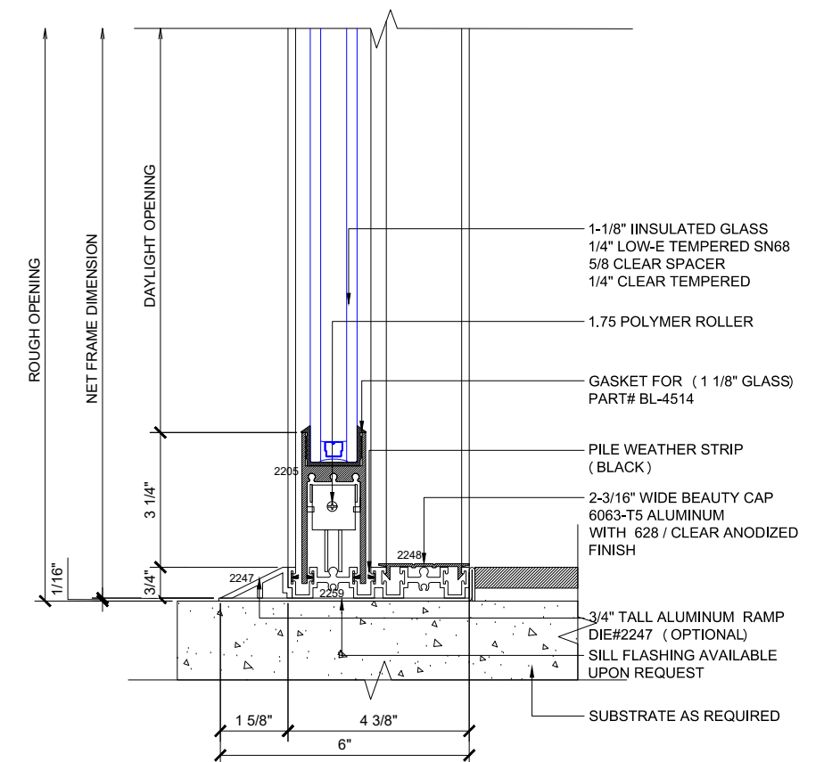
④ SILL (@SLIDER)
