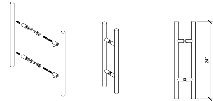
(F) 24 LADDER PULL RUBY SLIDING DOORS (OXO) SCALE: 6"=2'-0"
