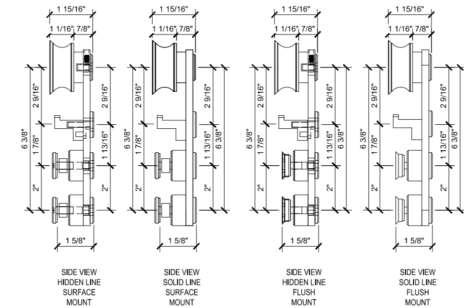
(A) PLHDSR ANTI-LIFT TOP ROLLER RUBY SLIDING DOORS (OXO) SCALE: 6"=1'-0"
