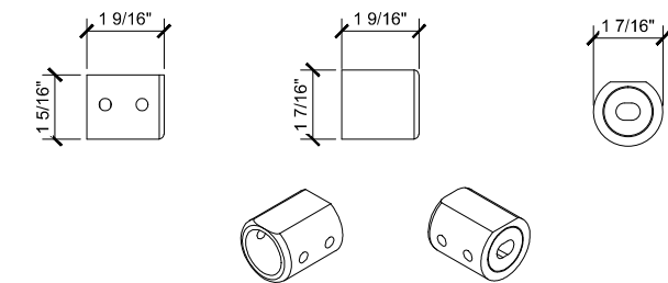
(H) PLTRACKFT RUBY SLIDING TUBE RUBY SLIDING DOORS (OXO) SCALE: 6"=1'-0"
