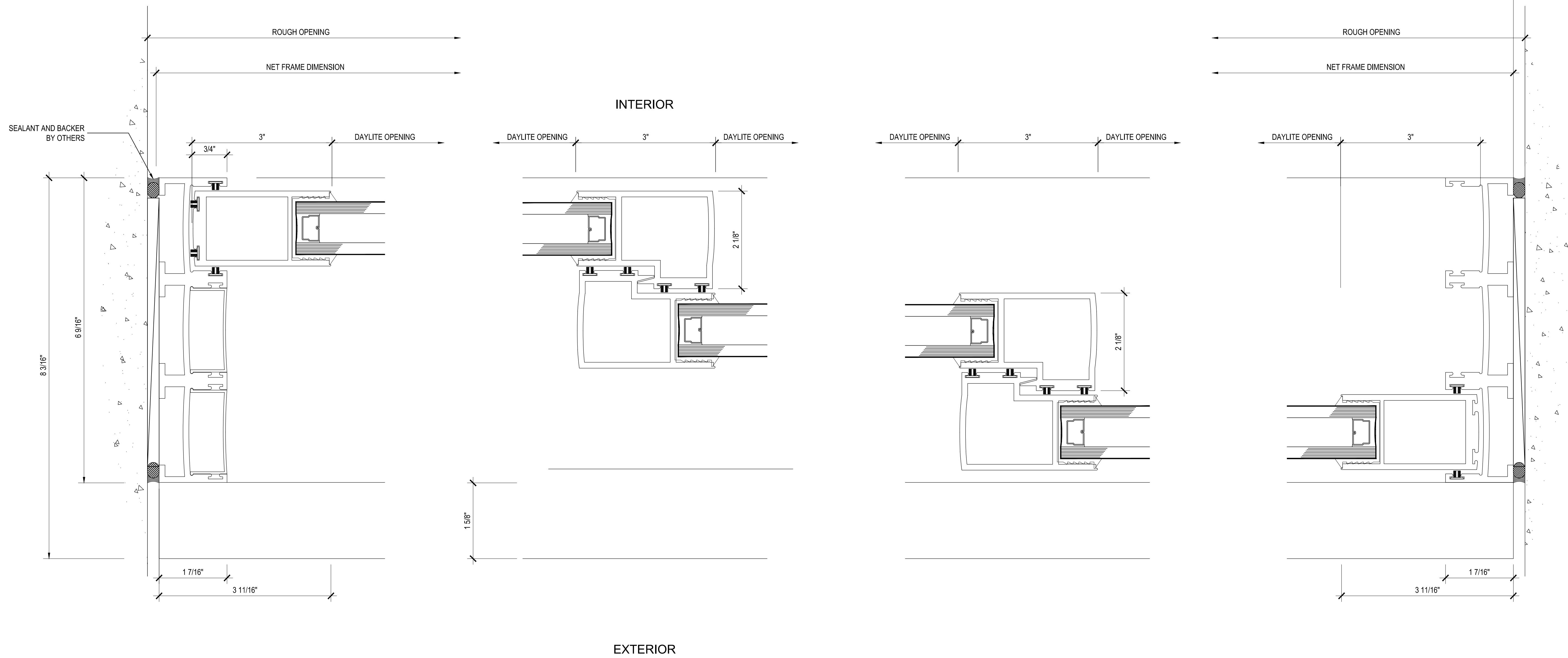
A Section @ Jambs Max-Slider Sliding Glass Door (XXO)
