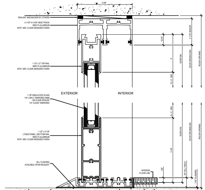
B Section @ (Fixed) Max-Slider Sliding Glass Door (XO)
