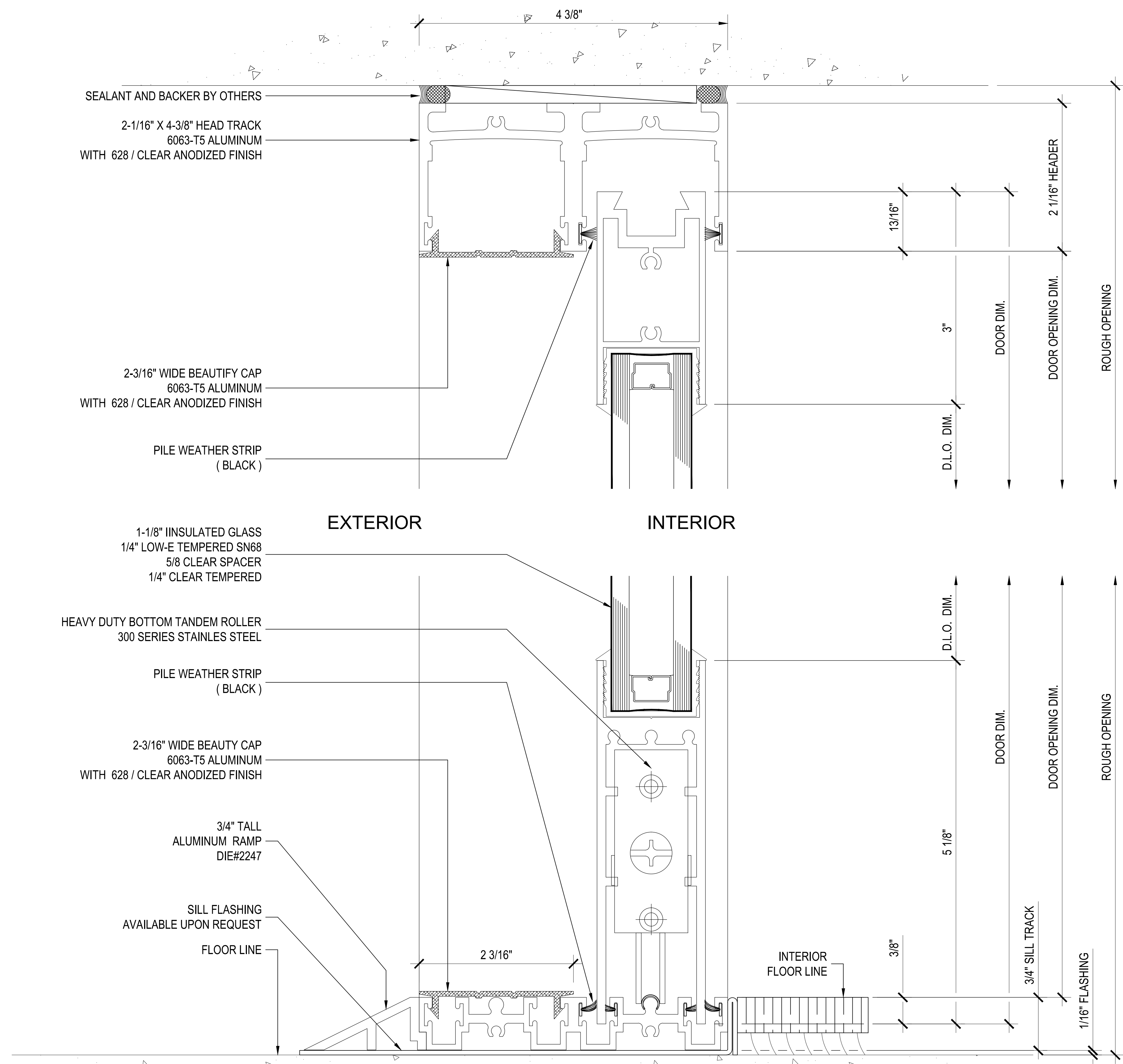
C Section @ (Slider) Max-Slider Sliding Glass Door (XO)
