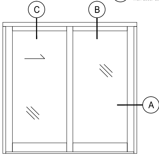
C Section @ (Slider) Max-Slider Sliding Glass Door (XO)
