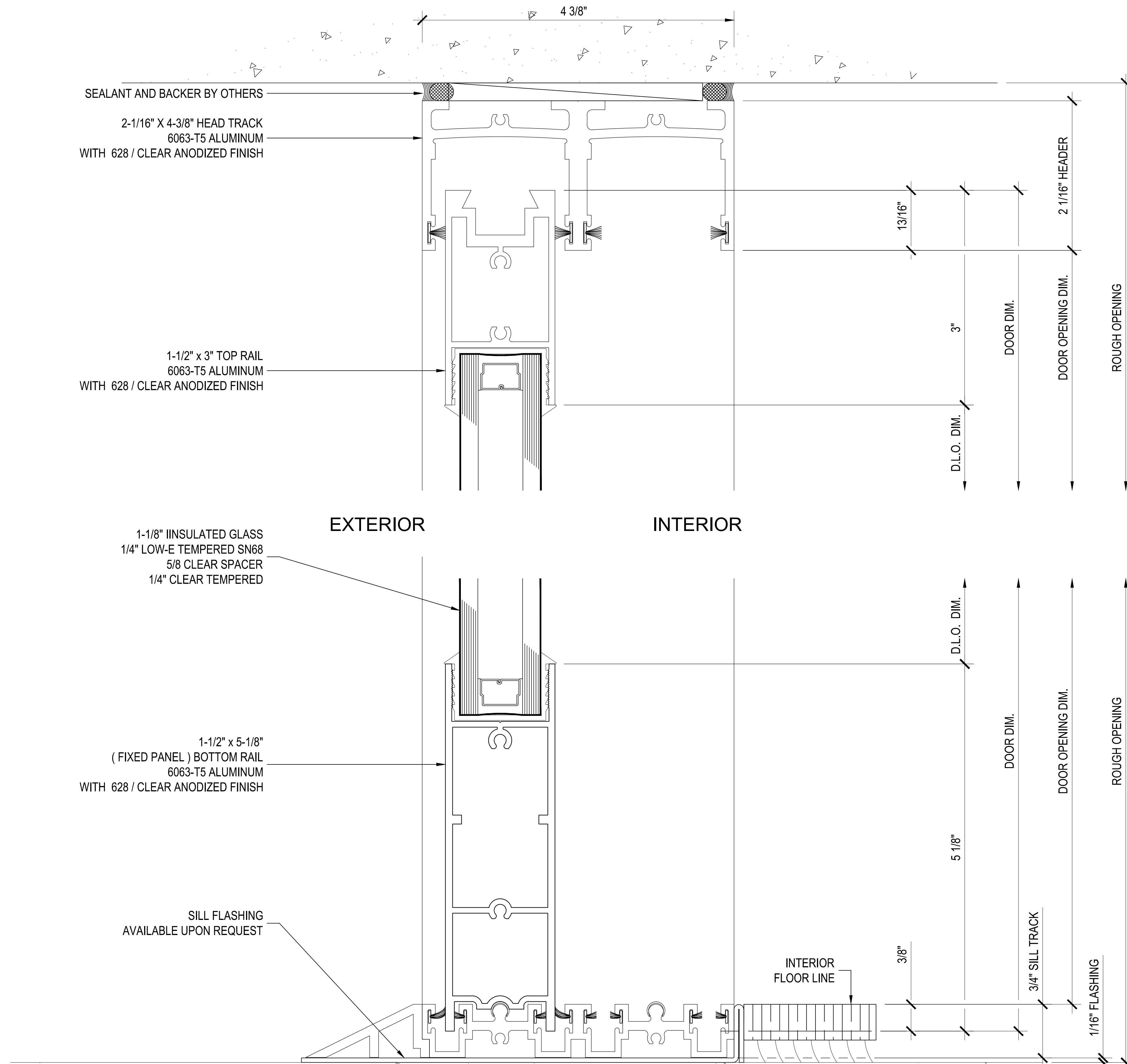
Section @ (Fixed) Max-Slider Sliding Glass Door (XO)
