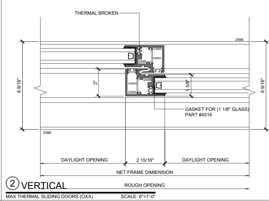
② VERTICAL MAX THERMAL SLIDING DOORS (OXX) SCALE: 6"=1'-0"
