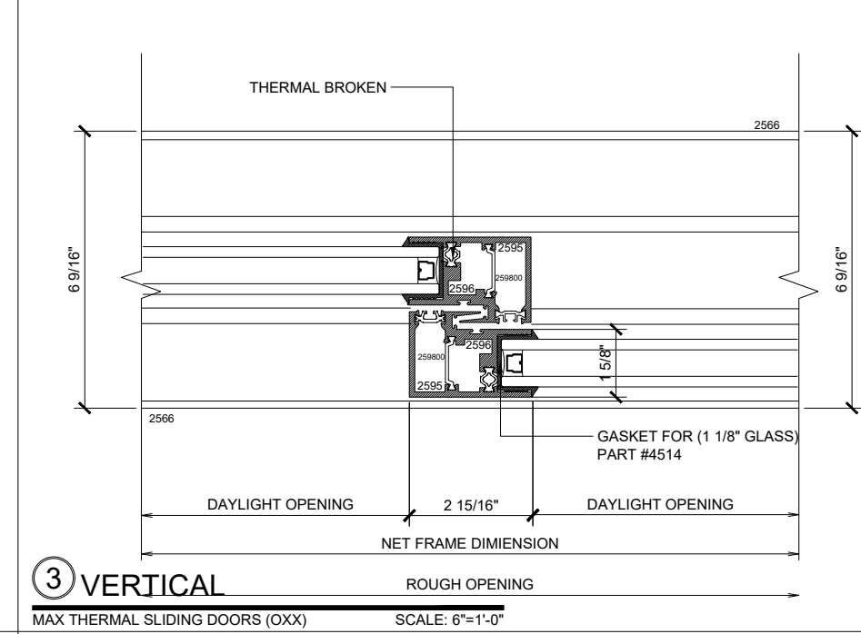
③ VERTICAL MAX THERMAL SLIDING DOORS (OXX) SCALE: 6"=1'-0"
