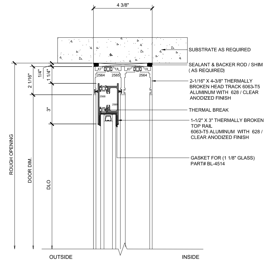
③ HEAD (@SLIDER)
