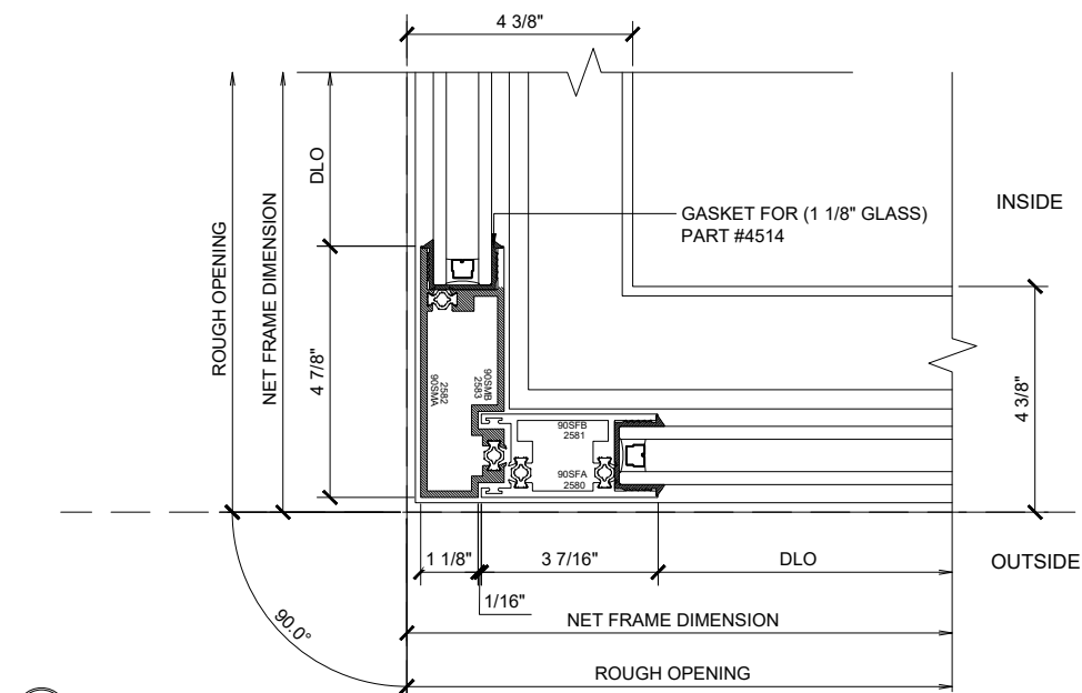
④ 90° CORNER DETAIL
