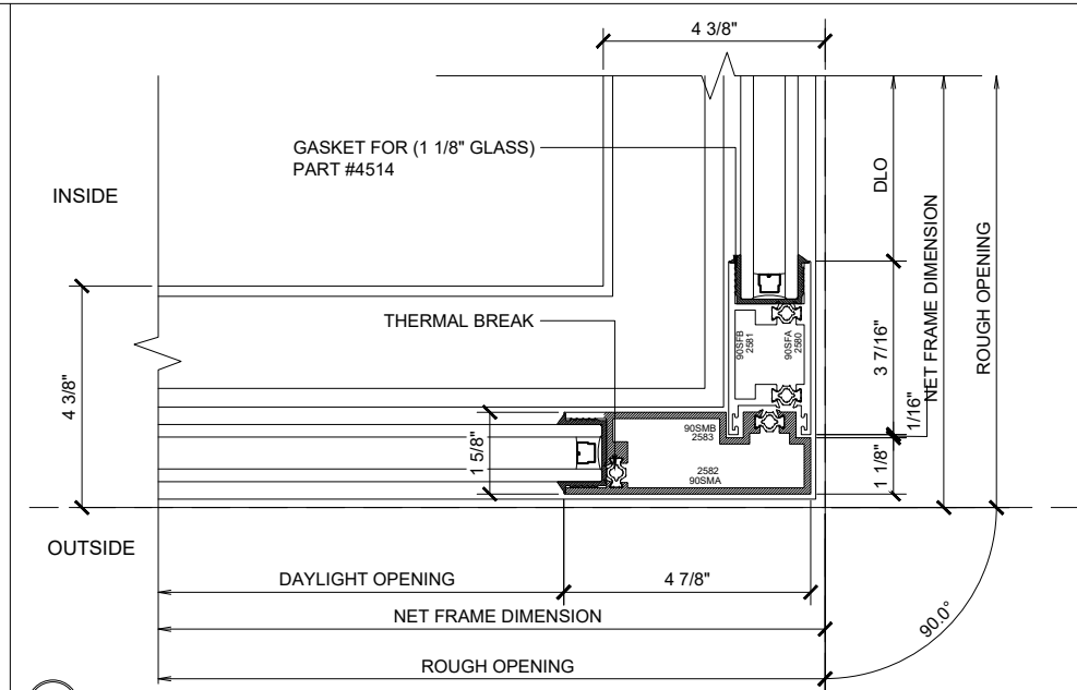
③ 90° CORNER DETAIL
