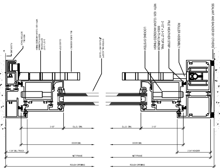
B Section @ (DOORS) PRL BI-FOLD DOOR SYSTEM
