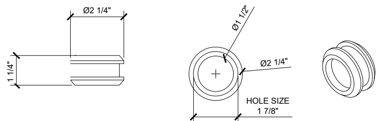
③ FINGER PULL
