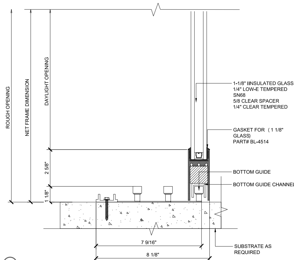
8 SILL (@SLIDER)
