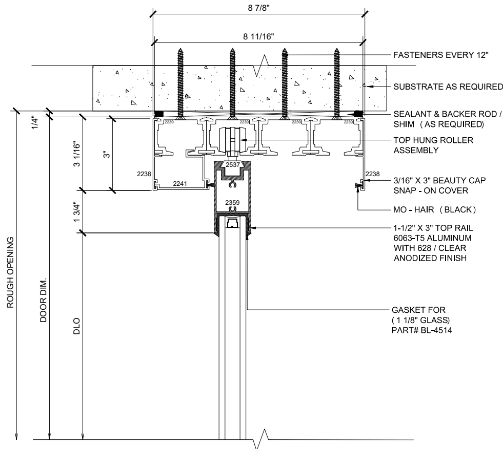
13 HEAD (@SLIDER) MAX SLIDING DOORS (OXXX-XXXO) SCALE: 6"=1'-0"
