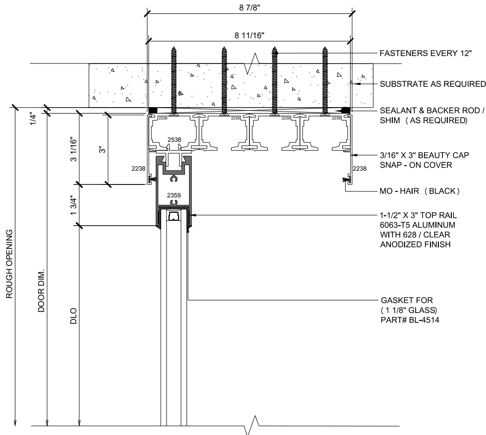
15 HEAD (@FIXED) MAX SLIDING DOORS (OXXX-XXXO) SCALE: 6"=1'-0"
