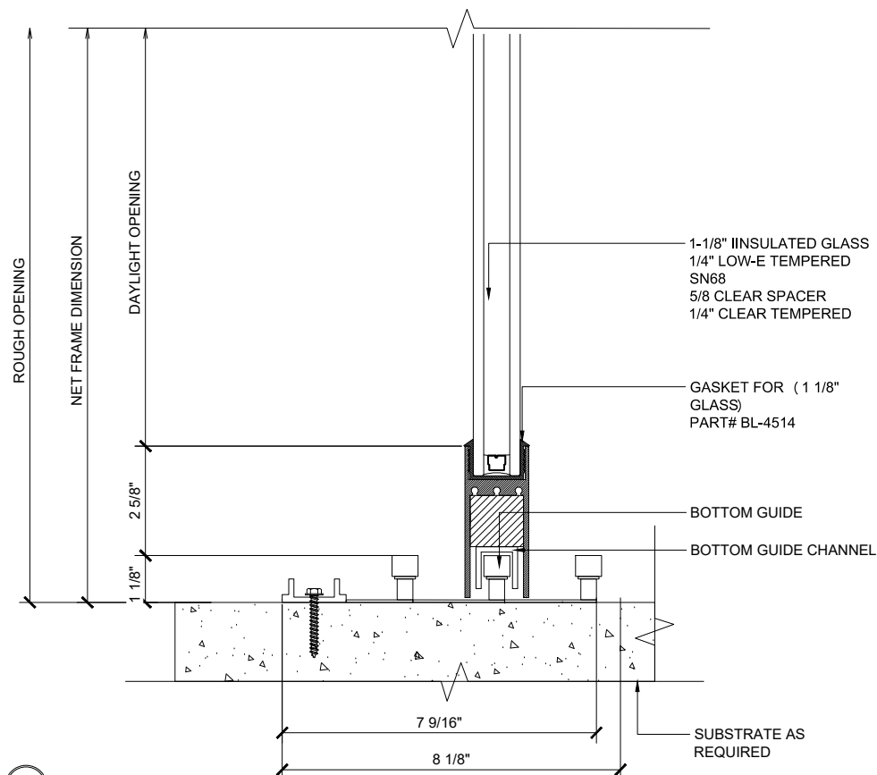
6 SILL (@SLIDER)
