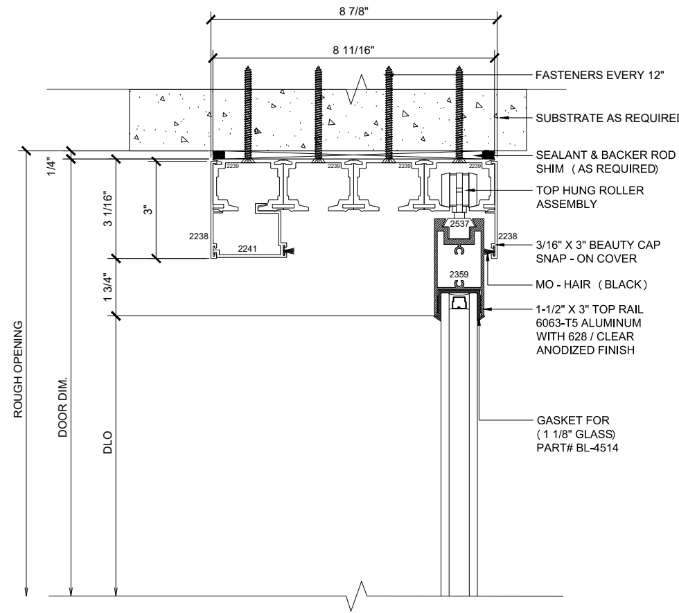
7 HEAD (@SLIDER)
