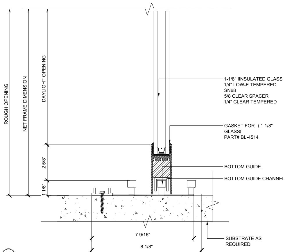
12 SILL (@SLIDER) MAX SLIDING DOORS (OXXX-XXXO) SCALE: 6"=1'-0"
