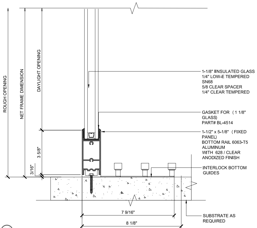
16 SILL (@FIXED) MAX SLIDING DOORS (OXXX-XXXO) SCALE: 6"=1'-0"
