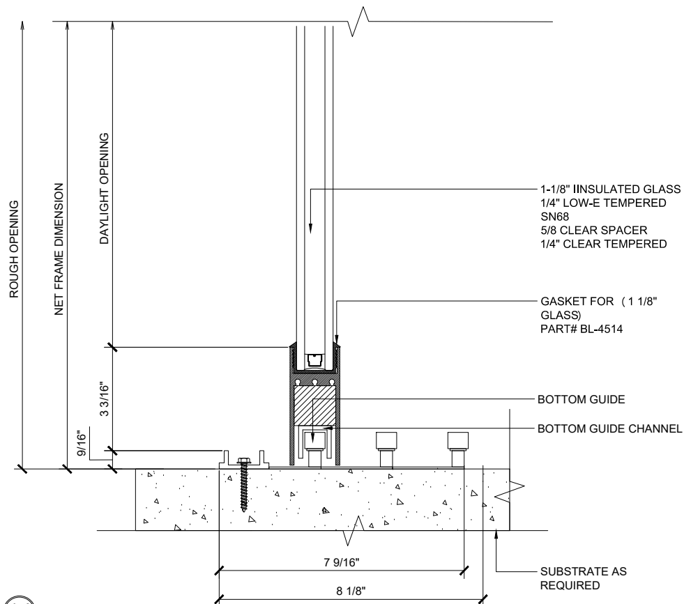
14 SILL (@SLIDER) MAX SLIDING DOORS (OXXX-XXXO) SCALE: 6"=1'-0"
