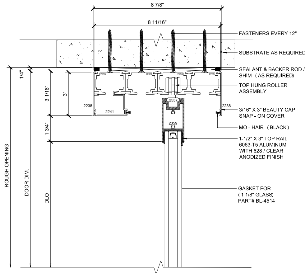
11 HEAD (@SLIDER) MAX SLIDING DOORS (OXXX-XXXO) SCALE: 6"=1'-0"
